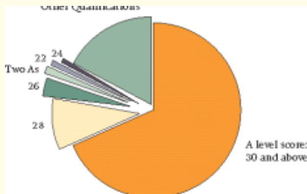
Distribution of scores of Post Q acceptances
